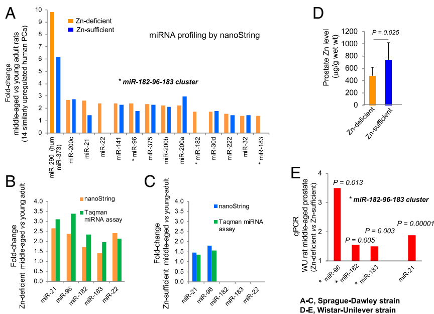
Fig. 3. Prostate miRNA expression profiling by the nanoString nCounter rat miRNA assay in Sprague-Dawley rats (A–C) and Wistar-Unilever rats (D and E) growing from young adult into middle age on a Zn-deficient diet or a Zn-sufficient diet. (A) Bar plot showing fold-change of 14 miRNAs up-regulated in Zn-deficient middle-aged vs. Zn-deficient young-adult prostates that are similarly up-regulated in human PCa compared with 11 such miRNAs up-regulated in Zn-sufficient middle-aged vs. Zn-sufficient young-adult prostates (cutoff: fold change \geq 1.4 , P < 0.05 , n = 6 rats per cohort). Asterisks denote up-regulation of the oncogenic miR-183-96-182 cluster. (B) Validation of five selected miRNAs (identified by the nanoString platform) in Zn-deficient middle-aged vs. Zn-deficient young-adult rat prostates by the TaqMan miRNA assay (with snoRNA as normalizer, measurements performed in triplicate, n = 8 rats per cohort). (C) Validation of five selected miRNAs (identified by nanoString platform) in Zn-sufficient middle-aged vs. young-adult rat prostates by the TaqMan miRNA assay (snoRNA as normalizer, measurements performed in triplicate, n = 8 rats per cohort). (D) Prostate Zn content (measured in micrograms per gram wet weight; mean \pm SD, n = 9 –11 rats per cohort). (E) Expression of the miR-183-96-182 cluster and miR-21 in prostates of Zn-deficient middle-aged Wistar-Unilever rats (qPCR, snoRNA as normalizer, assays performed in triplicate, n = 9 –12 rats per group). Data are expressed as fold-change in Zn-deficient vs. Zn-sufficient middle-aged rat prostates. All statistics are two-sided.
